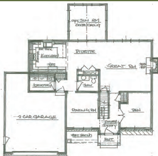
1 ST FLOOR PLAN RIVERA GREENS - THE MULBERRY #2200
